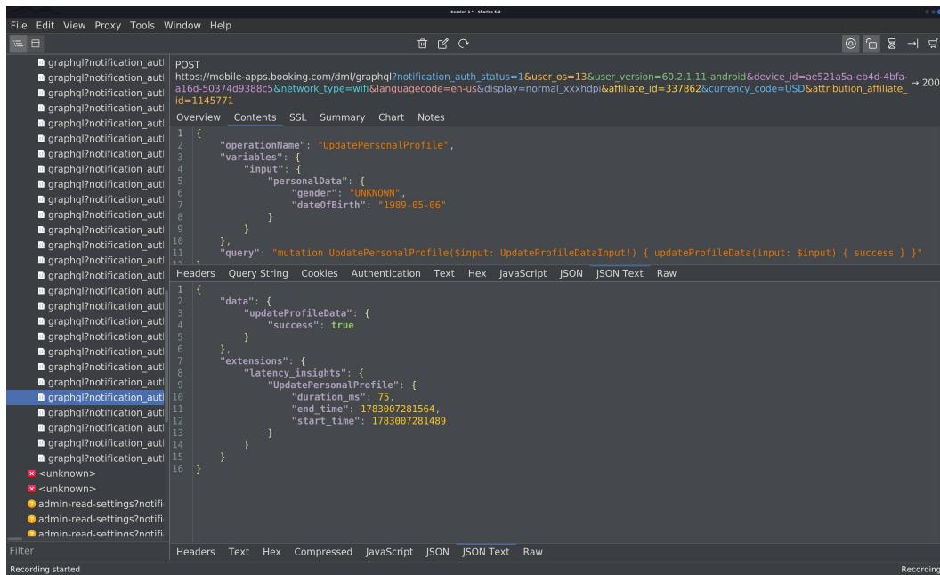
Figure 16: Executing UpdatePersonalProfile GraphQL mutation modifying authenticated user profile data
